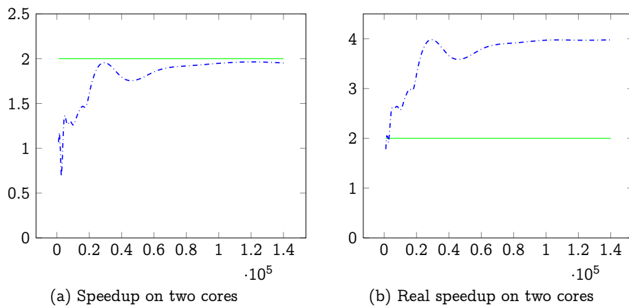
Figure 3.10: Benchmarking results of RowSplit with k = n_2/p+1 + 1 -\cdot-\cdot- on M_1 against input size n_2 for fixed n_1 = 1000 . Note the optimum -\cdot-\cdot- .
